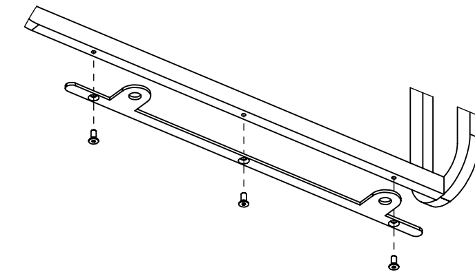
DETAIL G SCALE 1 : 5
