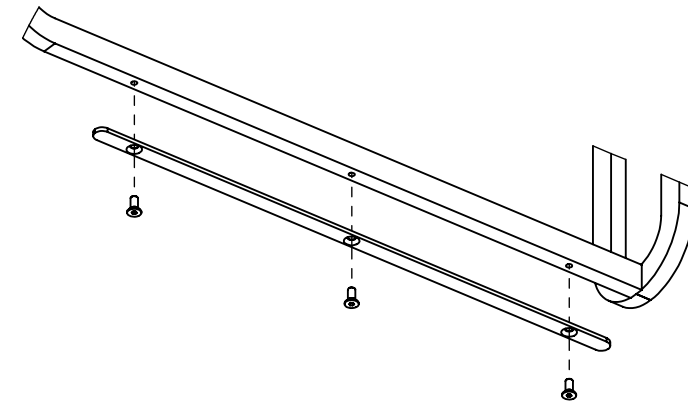
DETAIL F SCALE 1 : 5
